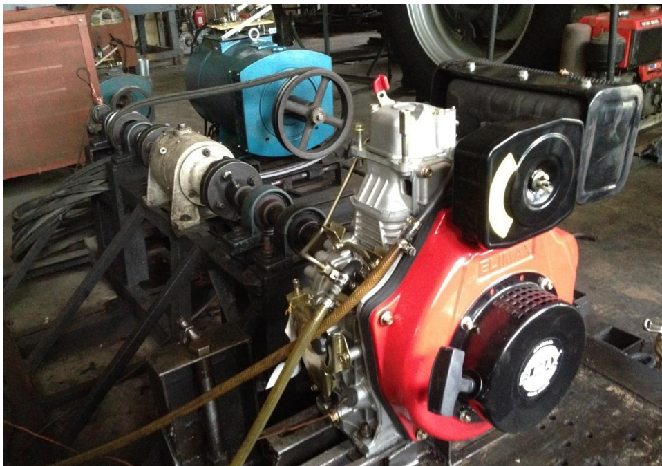
Figure 2. Test set-up of the ELIMAX EM178F/S Diesel Engine
