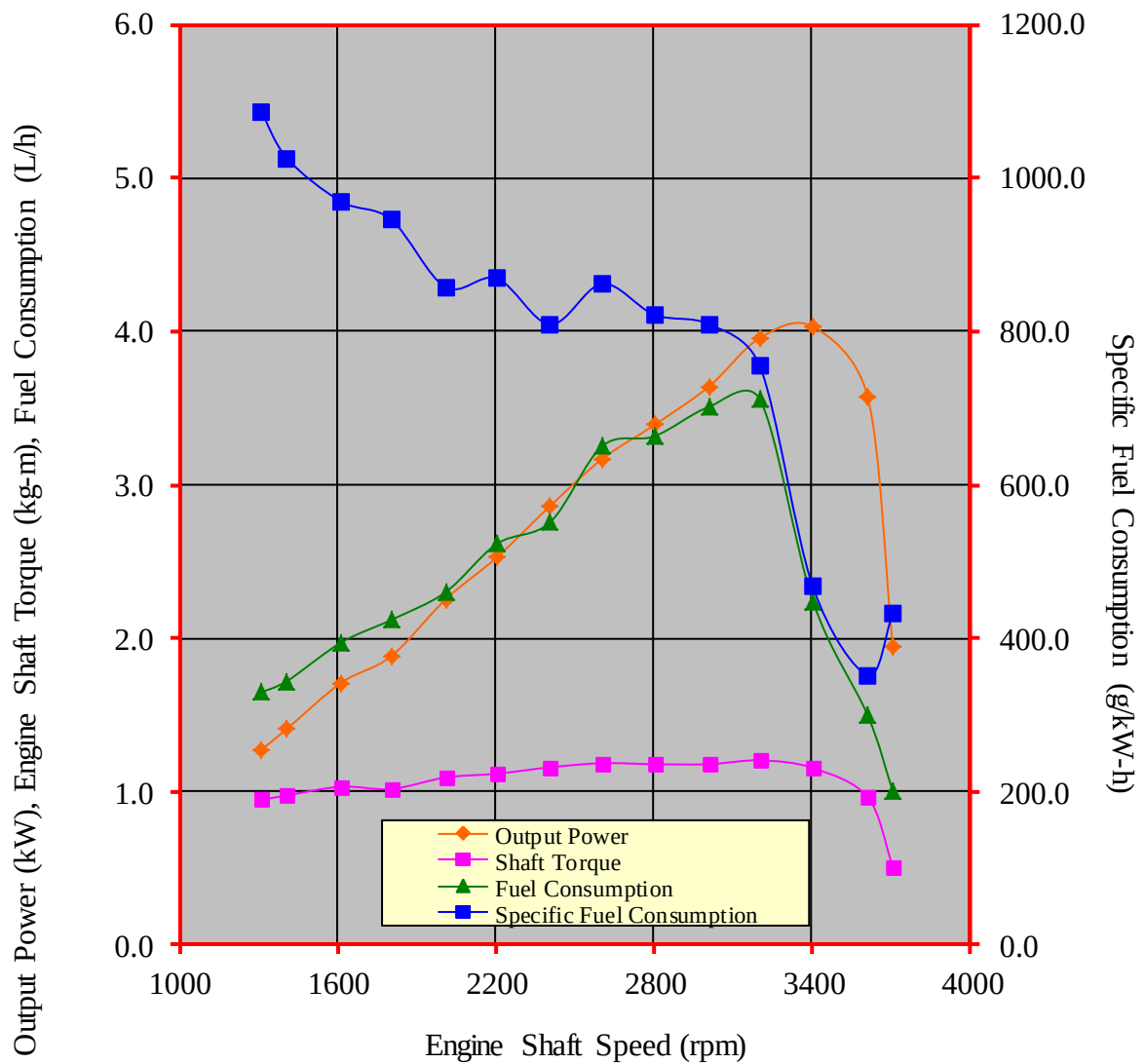
Figure 3. Performance characteristic curves of the ELIMAX EM178F/S diesel engine
