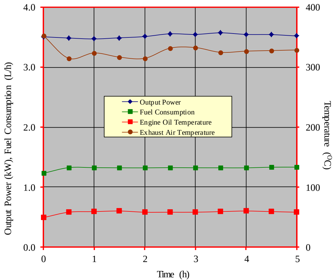
Figure 4. Performance characteristic curves during the continuous running test ELIMAX EM178F/S diesel engine
